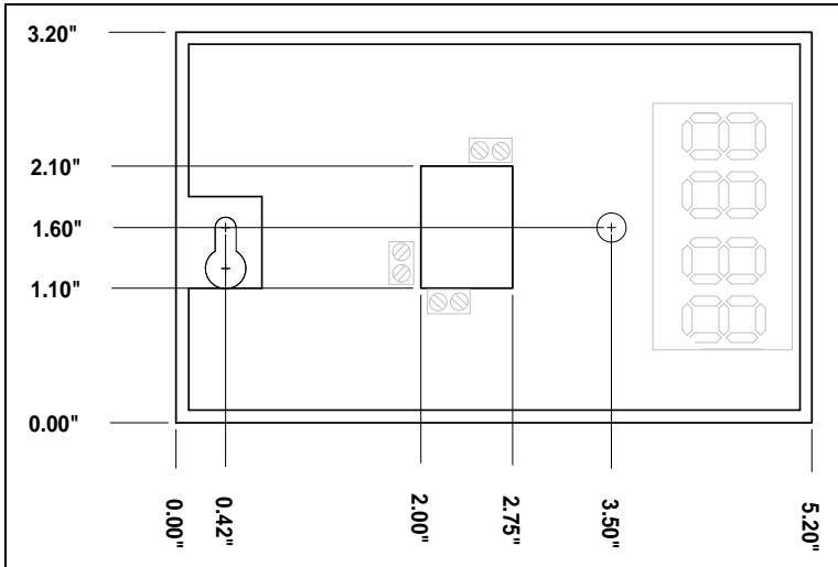
Figure 1: Kele Model CD-AW Mounting Dimensions
